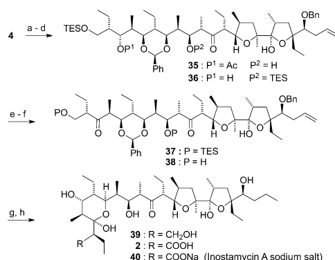
Scheme 6. Reagents and conditions. a) \text{TMP}\cdot\text{HBr} , n\text{BuLi} , THF, -78^\circ\text{C} , then 3 in THF, -78^\circ\text{C} , 92%; b) TESOTf, 2,6-lutidine, \text{CH}_2\text{Cl}_2 , -78^\circ\text{C} , 94%; c) PPTS, EtOH, -20^\circ\text{C} , then \text{K}_2\text{CO}_3 , -20 to 25^\circ\text{C} ; d) \text{TESCl} , \text{Et}_3\text{N} , \text{CH}_2\text{Cl}_2 , -78^\circ\text{C} , 94% (over 2 steps); e) AZADO, \text{PhI}(\text{OAc})_2 , \text{CH}_2\text{Cl}_2 , Py, 0 to 25^\circ\text{C} , 92%; f) \text{Et}_3\text{N}\cdot 3\text{HF} , MeCN, 25^\circ\text{C} , 92%; g) \text{H}_2 , 10% Pd/C, Amberlite IRA-67, EtOH, 25^\circ\text{C} , 94%; h) TEMPO, \text{NaOCl} , pH 6.7 phosphate buffer, \text{H}_2\text{O} , MeCN, 25^\circ\text{C} , then aq \text{Na}_2\text{S}_2\text{O}_3 , aq \text{NaHCO}_3 , 84%.
