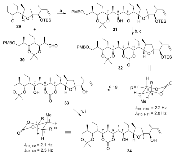
Scheme 5. Reagents and conditions. a) \text{TMP}\cdot\text{HBr} , n\text{BuLi} , THF, -78^\circ\text{C} , then 30 in THF, -78^\circ\text{C} , 90%; b) \text{Me}_4\text{NBH}(\text{OAc})_3 , AcOH, MeCN, 0 to 25^\circ\text{C} , 80%; c) triphosgene, Py, \text{CH}_2\text{Cl}_2 , -78 to 0^\circ\text{C} , 90%; d) \text{Et}_3\text{N}\cdot 3\text{HF} , MeCN, 40^\circ\text{C} , 95%; e) DDQ, pH 7 phosphate buffer, \text{CH}_2\text{Cl}_2 , 0^\circ\text{C} , 88%; f) 1 M aq HCl, THF, 25^\circ\text{C} , 94%; g) PPTS, \text{Me}_2\text{C}(\text{OMe})_2 , \text{CH}_2\text{Cl}_2 , 0^\circ\text{C} , 93%; h) \text{K}_2\text{CO}_3 , MeOH, 25^\circ\text{C} , 92%; i) triphosgene, Py, \text{CH}_2\text{Cl}_2 , -78 to 0^\circ\text{C} , 89%, \text{TMP} = 2,2,6,6 -tetramethylpiperidine.
